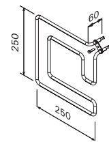
ZTA-10 1000W/400V WH(K)4, WH(K)5
