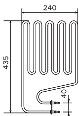
ZSP-240 2150W/230V K11G/S PO11
