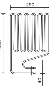
ZSP-250 2500W/230V F15, F16,5, K13.5G/S, K15G/S PO165
