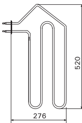
ZSF-20 1333W/230V AF4
