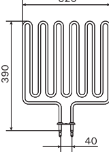
ZSL-313 2000W/240V K9, K10,5, K12, L26
