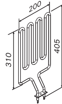
ZSN-160 1800W/230V D29EE, D36/E, D36EE
