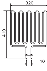
ZSK-720 3000W/230V KIP90E, M90E KV90SE/A
