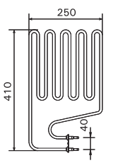
ZSS-110 1500W/230V T9, T10,5, F10,5 T7C/A-T9C/A, K11G/S, K13.5GS PO11
