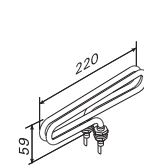
ZSB-571 2000W/230V BC60SE(A), BC90SE(A)
